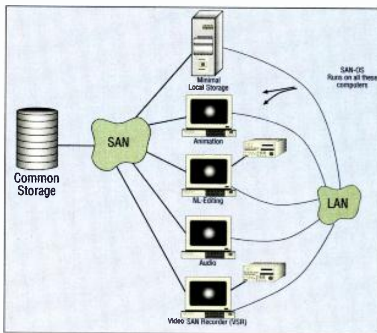
Figure 1. The SAN provides a direct link between shared storage and every video workstation and VSR in the facility, allowing everyone to use the same disks at the same time.
